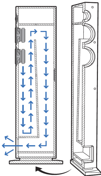
MK442T Cross Section
